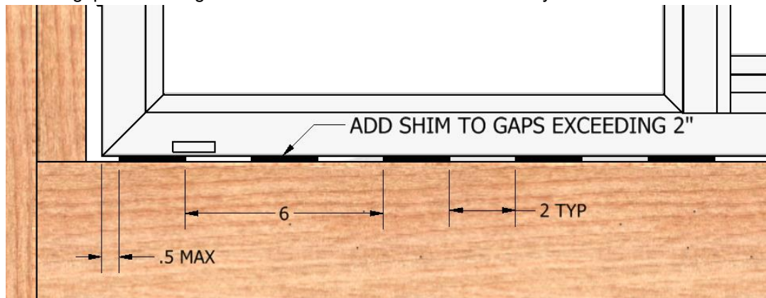
SILL VIEW
