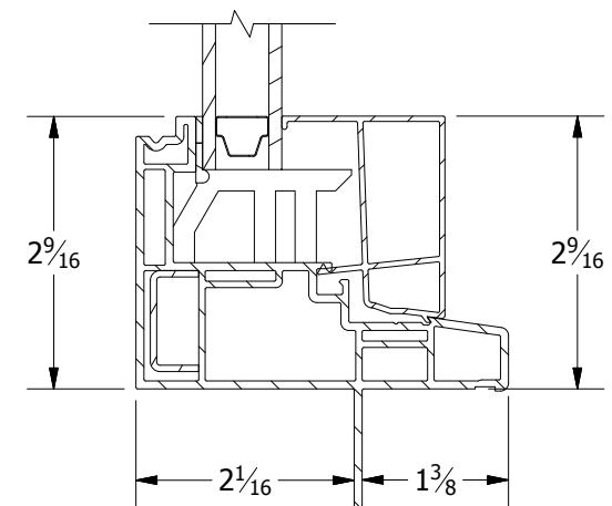
SECTION NARROW T-BAR SCALE 1 / 2
