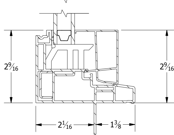
SECTION WIDE T-BAR SCALE 1 / 2
