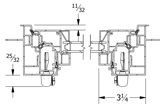
SECTION C-C SCALE 1 / 4
