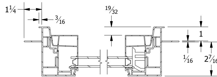
SECTION B-B SCALE 1 / 4
