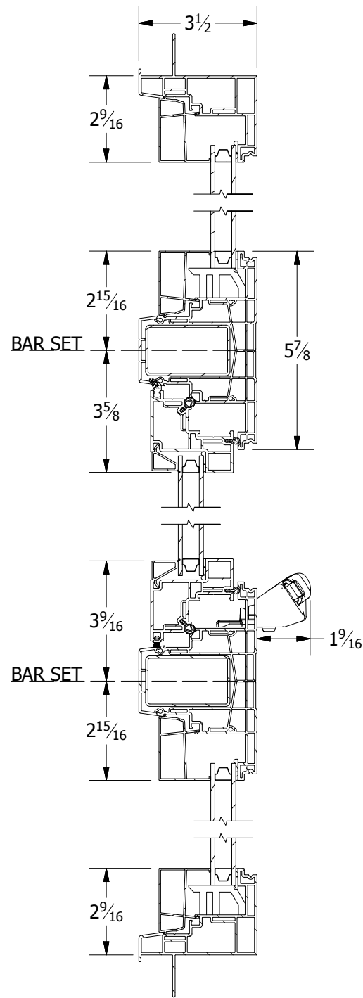
SECTION A-A SCALE 1 / 4
