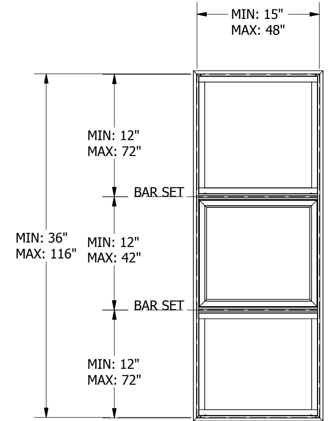
EXTERIOR SCALE 1 / 32
